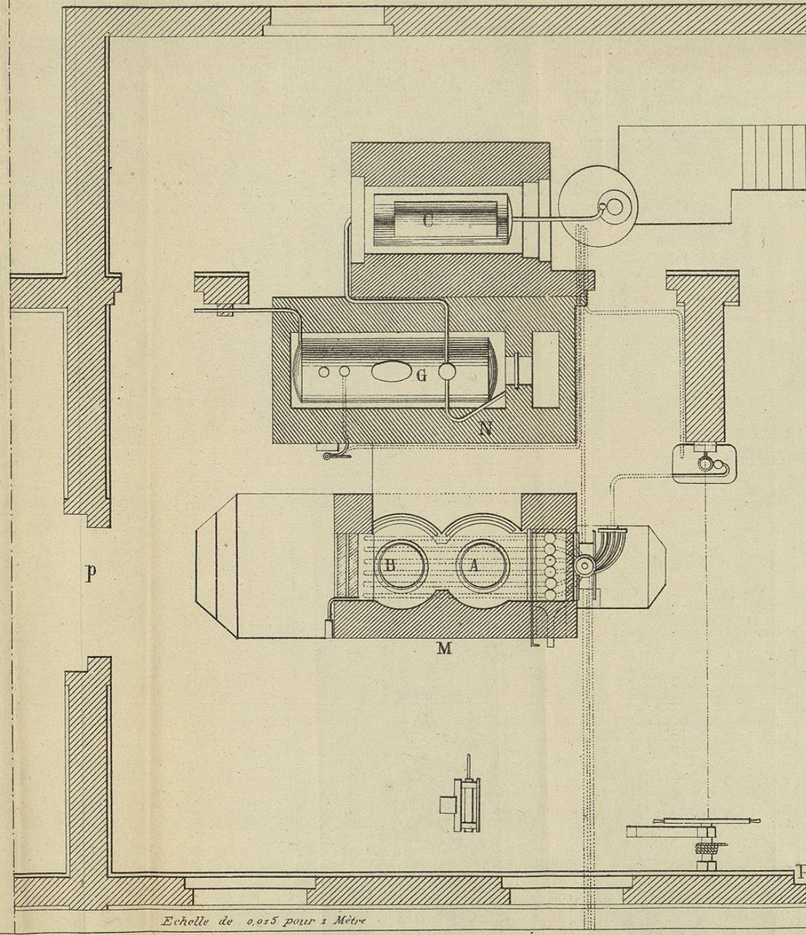
Fig 2. Plan
