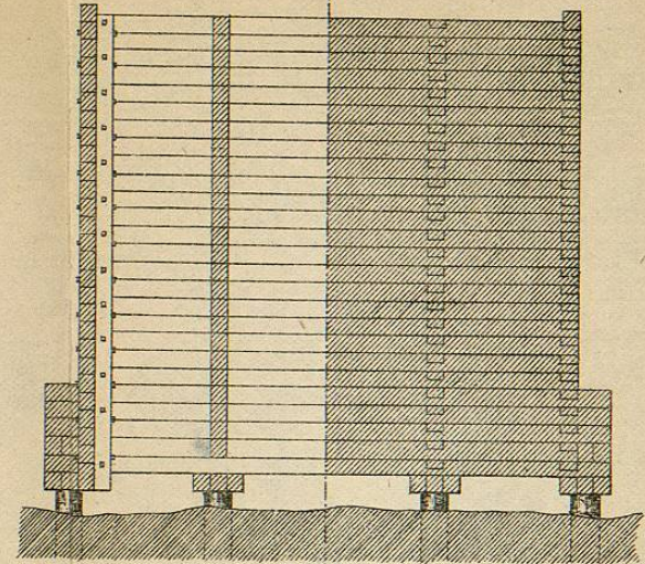
Section on GHIJ
