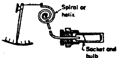
FIG. 9. Filled-system thermometer.
