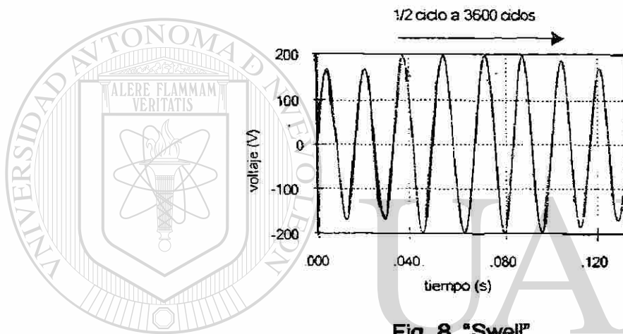
Fig. 8. “Swell”
