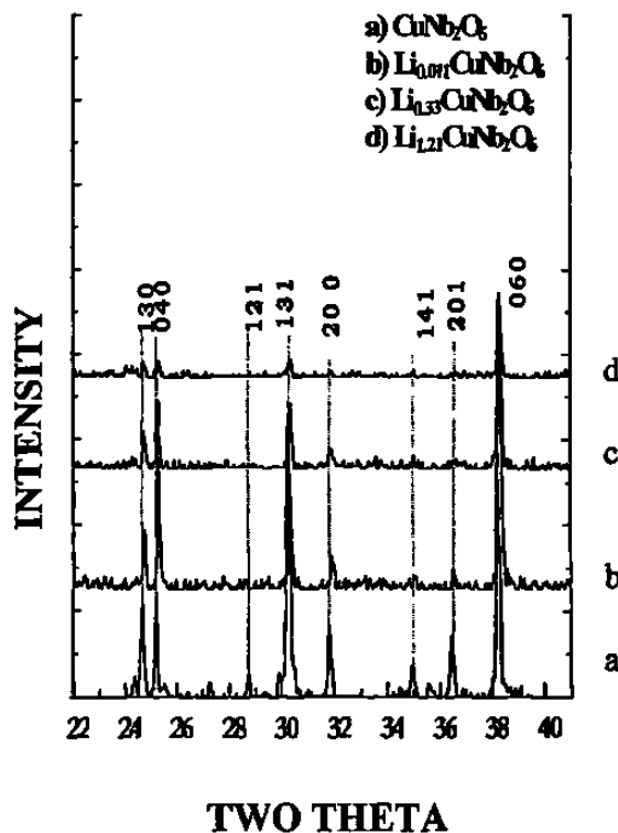
Fig. 3. X-ray diffraction patterns obtained from an in situ experiment using \text{CuNb}_2\text{O}_6 as the active material.
