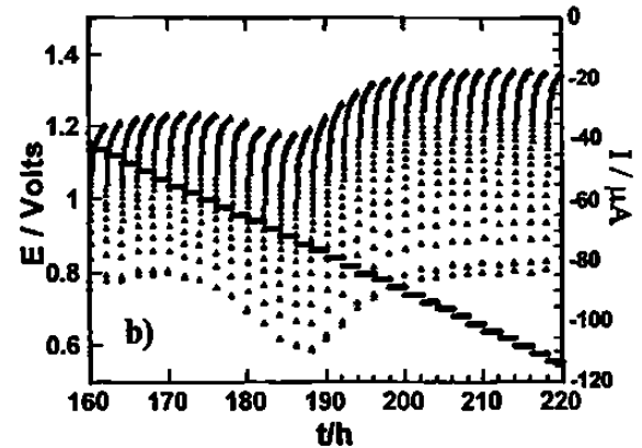
Fig. 4. A chronoamperogram showing details of the kinetics of lithium insertion into \text{CuNb}_2\text{O}_6 (a) at the first reduction process, and (b) when lithium diffusion determines the insertion reaction.
