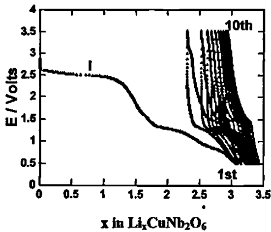
Fig. 2. Voltage vs. composition for successive charge–discharge cycles of a cell using \text{CuNb}_2\text{O}_6 as active material.
