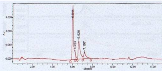
Chaparrina
