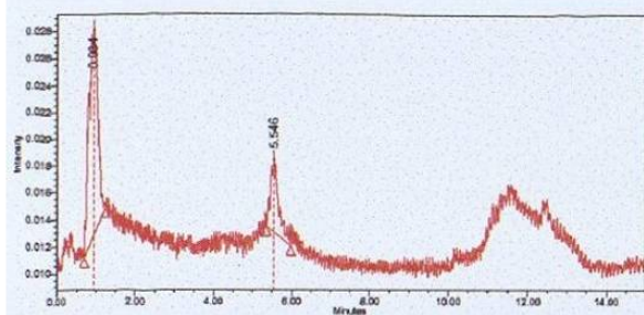
Chaparrina
