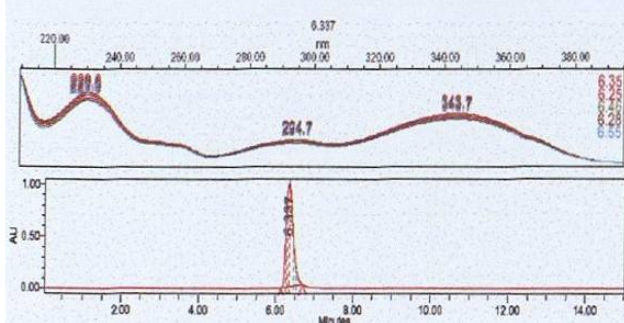
Kokusagenina
