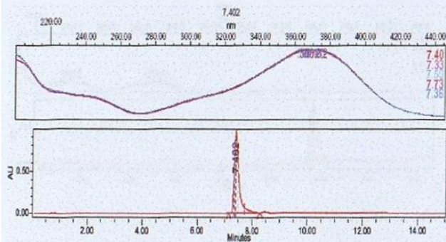
Kokusagenina
