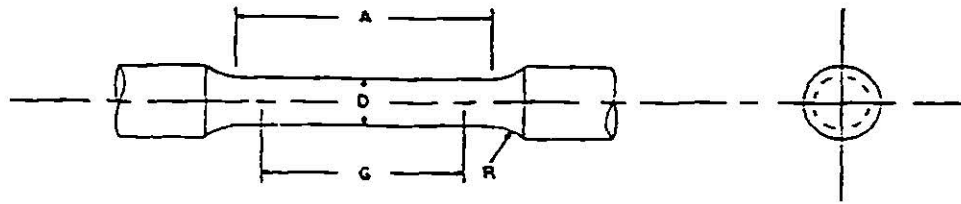
Dimensions, mm
