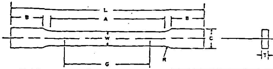
Dimensions, mm
