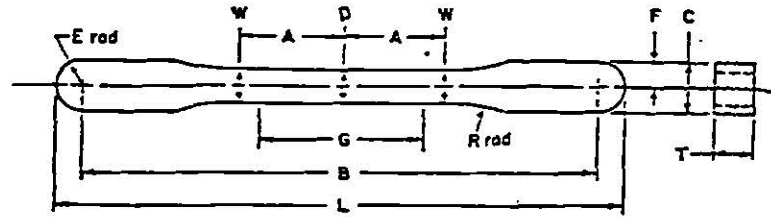
Dimensions, mm
