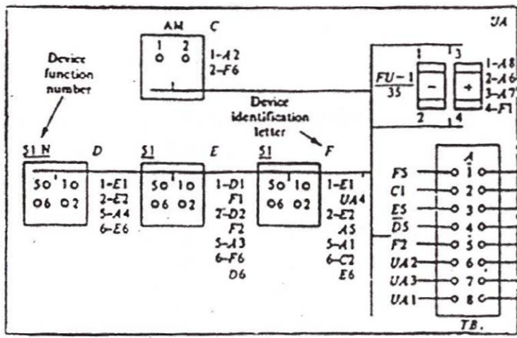
Panel-back view
