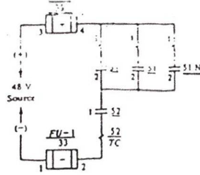
(a) Elementary control diagram
