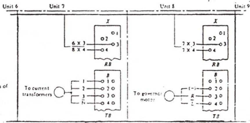
(c) Interconnection diagram
