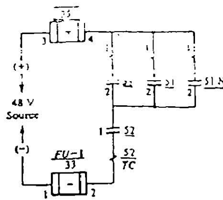
(a) Elementary control diagram
