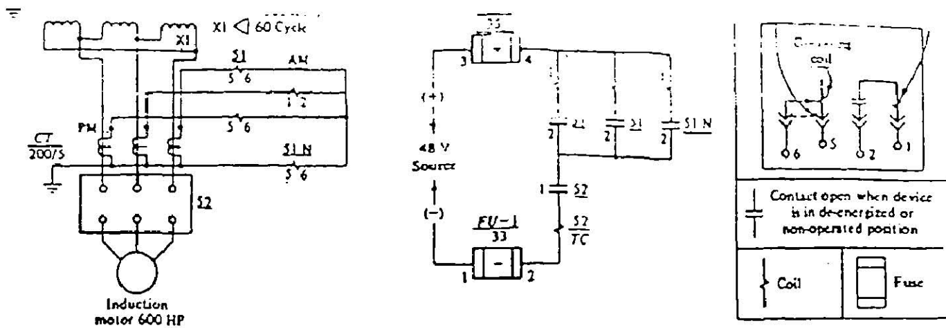
(a) Elementary control diagram
