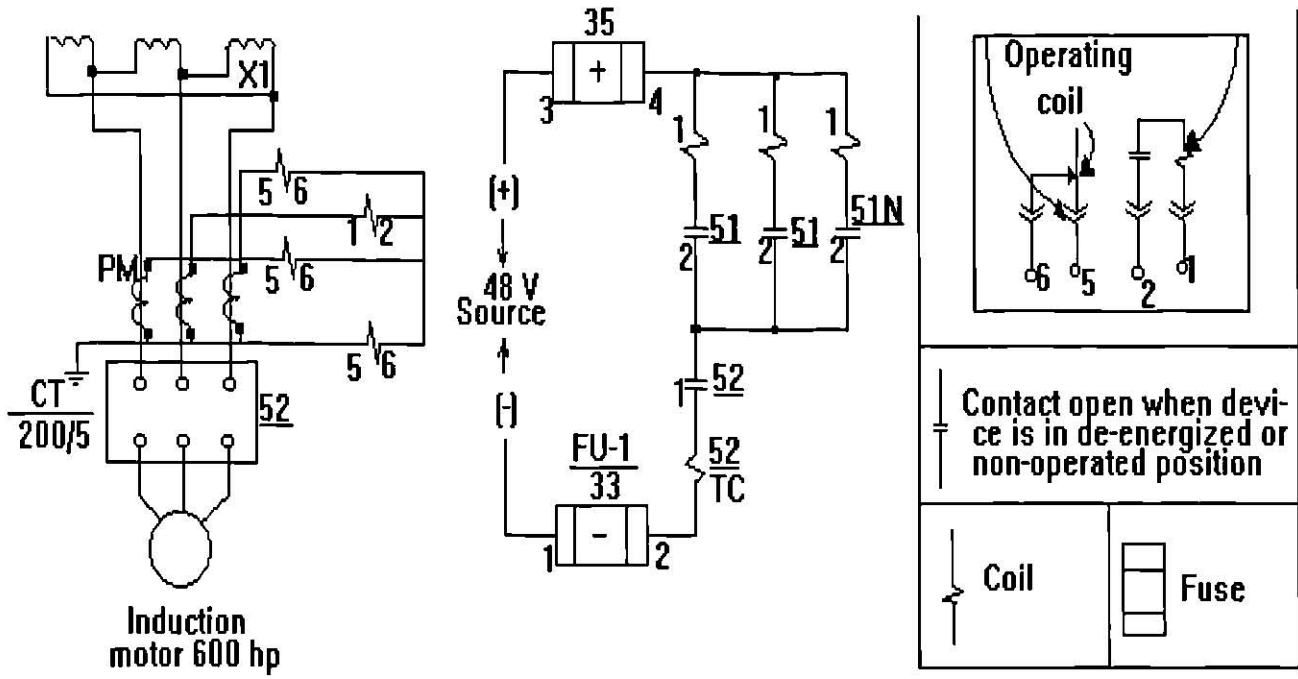
[a] Elementary control diagram
