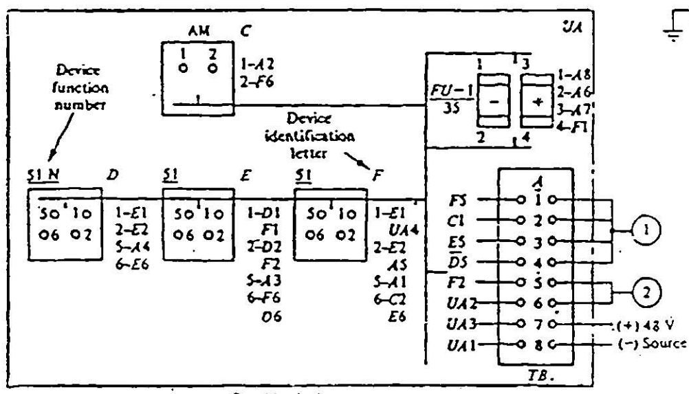
Panel-back view
