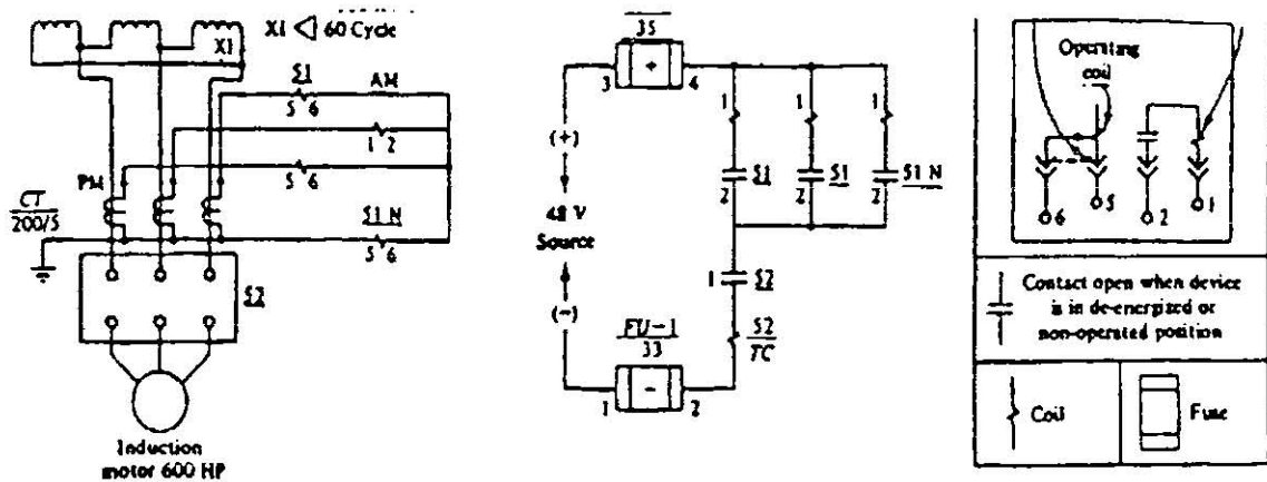
(a) Elementary control diagram
