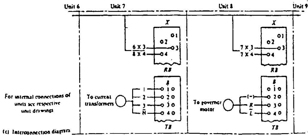
(c) Interconnection diagrams
