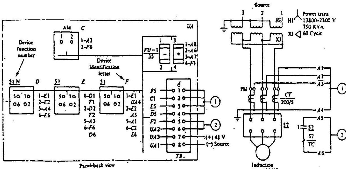
(b) Connection diagram
